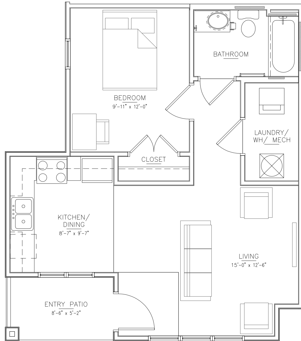
UNIT TYPE A - 1BR/1BA
